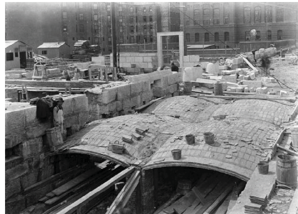
Fig. 3. a) Rafael Guastavino standing on a newly built arch during construction of the Boston Public Library, Boston, Massachusetts, 1889. [10] b) Guastavino Rib and Dome System, New York, 1902. [11]
