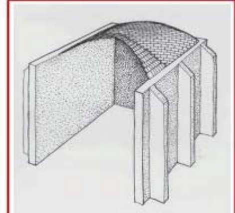
Fig. 3. Three methods of brick vault construction [7]: a) Northern European vaults require extensive wooden centering; b) pitched brick vaults, built in North Africa and Mexico, eliminate the need for centering; and c) Mediterranean tile vaults may be constructed without centering.
